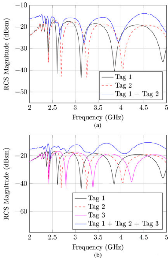
Fig. 3. Multi-tag interference simulation study for: (a) two tags with different codes. (b) Three tags with different codes.
