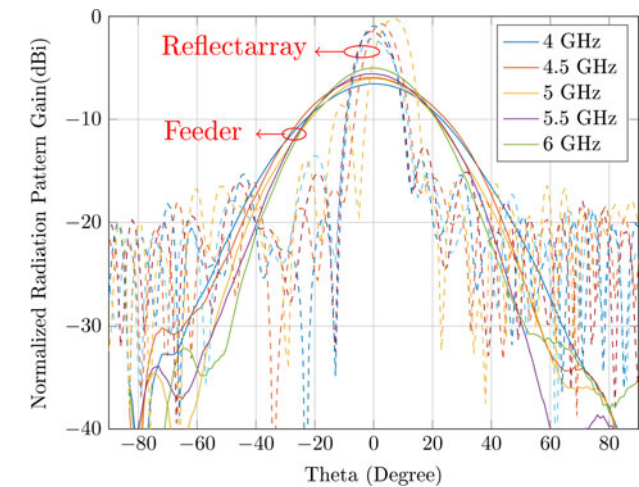
Fig. 13. The measured radiation patterns of the UWB feeder vs the UWB RA antenna.
