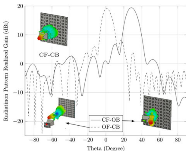
Fig. 9. Simulated realized gain patterns for the CFOB and OFCB configurations at 5 GHz.
