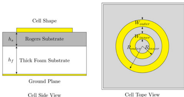
Fig. 6. Fixed beam RA antenna basic cell configuration.
