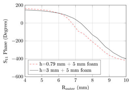
Fig. 8. UWB RA cell reflection phase with the outer ring radius at 5 GHz and the other cell dimensions are in relation to R_{outer} .
