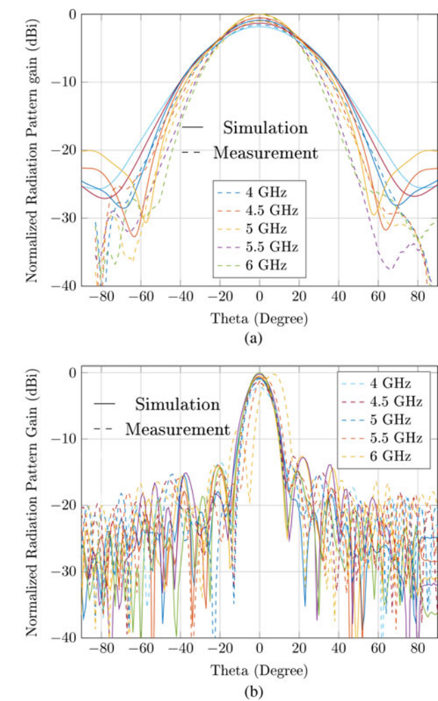
Fig. 12. Radiation patterns simulation and measurements: (a) Feeder simulated and measured radiation patterns. (b) Complete UWB RA antenna simulated and measured radiation patterns .
