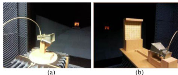
Fig. 11. Measurements setup: (a) Feeder measurement setup. (b) Complete RA antenna measurement setup inside AC.
