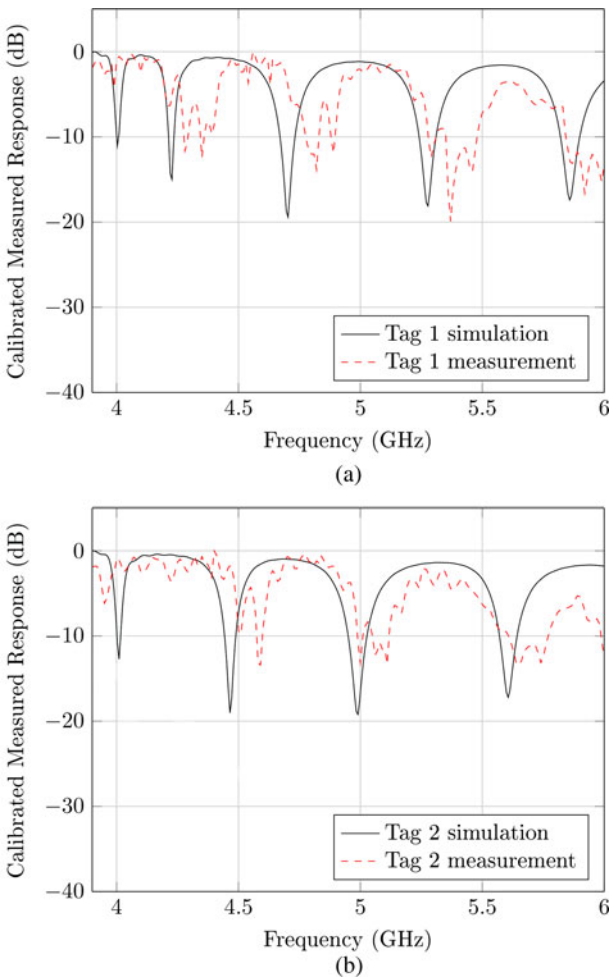
Fig. 15. Testbed simulation and measurement results for the first tag with code (11010101) and for the second tag (10101010).
