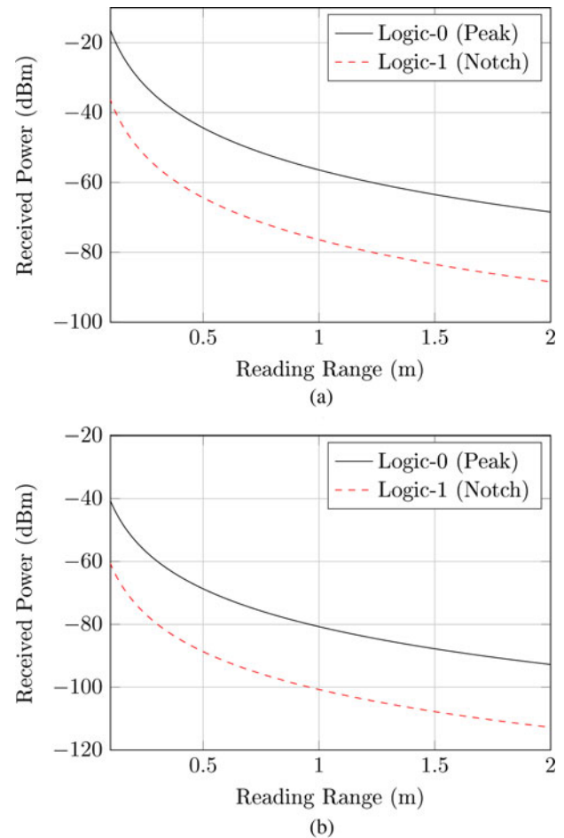
Fig. 4. Theoretical reading range as a function of the received power at 5 GHz in case of: (a) UWB transmission with -41.3 dBm/MHz, (b) frequency sweeping interrogation with 0 dBm/50 MHz.
