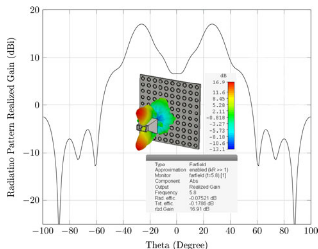
Fig. 10. Simultaneous dual-beam configuration with two beams directed at \phi = 90^\circ , \theta = 30^\circ and \phi = 90^\circ , \theta = -30^\circ .
