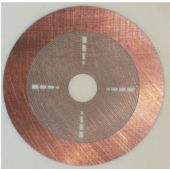
Fig. 1. NPM RCS manufactured tag.
