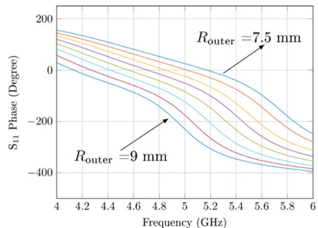
Fig. 7. Reflection phase variation with frequency for different outer ring radius.
