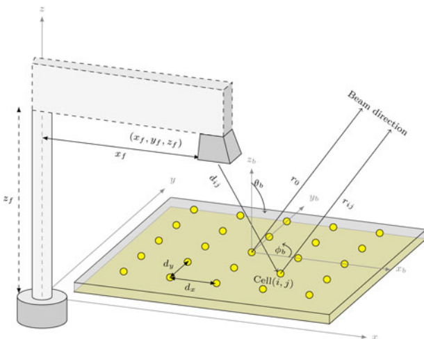
Fig. 5. RA building blocks.
